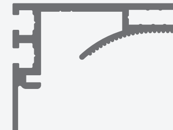
TECHO 45 44.3x34.6mm
