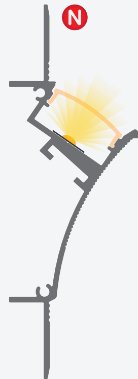
TIJUANA 34.8x98mm
