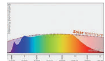
Luminous spectrum with Sevilla ecoled
