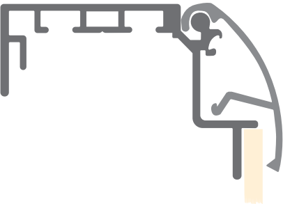
scale profile 1:1
