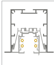
KRAKOVIA with tray and "Global" 3-phase rail
