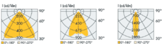
Extra Wide 90° Ref: 46.010 Wide 60° Ref: 46.004 Narrow 30° Ref: 46.005
