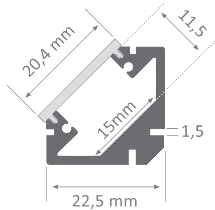
Difusor XL LP01/1D: blanco opal LP01/2D: glaseado LP02/1D: transparente PVP: 5,18€
